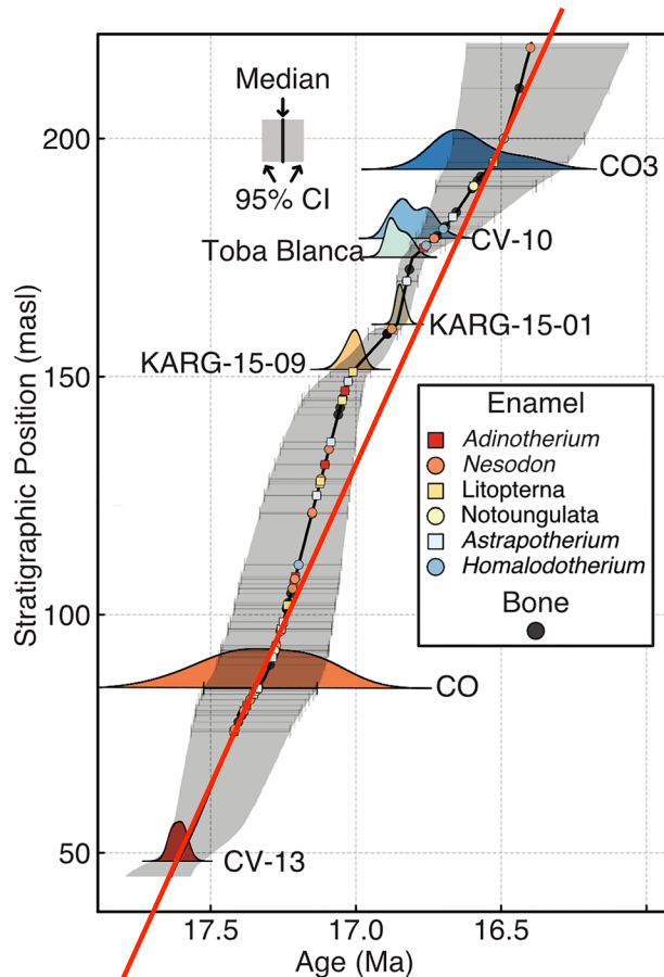
Figure 2. Age-depth model for a composite section of the Cañadón de las Vacas and Rincón del Buque localities. Colored areas with tails are the probability distribution functions for each marker tuff (modified from Trayler et al., 2020). Colored dots and error bars indicate the median age and uncertainty expressed as 95% credible intervals (CI) of fossil bone and enamel samples. See supporting information for precise stratigraphic positions for all fossil samples.
